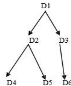
Figure 1: OpenDependency Structure
